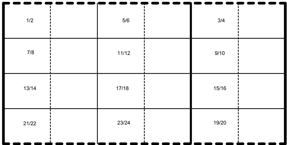
SOLAR PANEL
